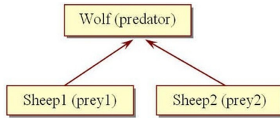
Fig.8 The simple food-web corresponding to the new “System Modeler Food-web without grass” Model.
